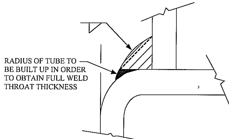
FIGURE 6.1 BUILD UP RADIUS WELD
