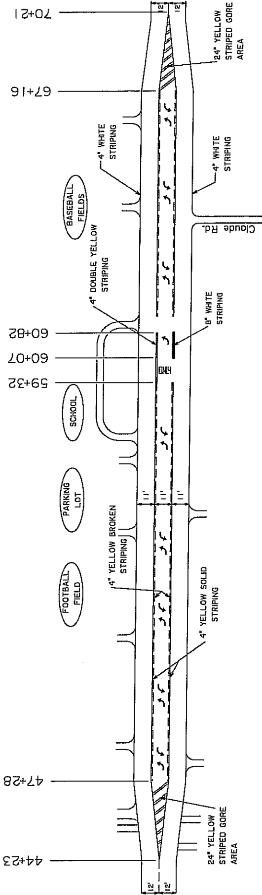
Left Turn Lane Layout
