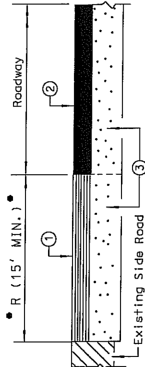
BASE AND SURFACING DETAIL (SECTION H-H)
