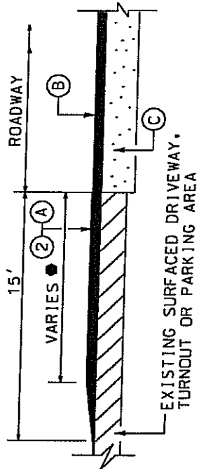
SURFACING DETAIL (SECTION H-H) TO APPLY FOR EXISTING SURFACED TURNOUTS.
