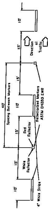
LAYOUT B To Be Used for Lane Line Between Lanes of Traffic Traveling in the Same Direction
