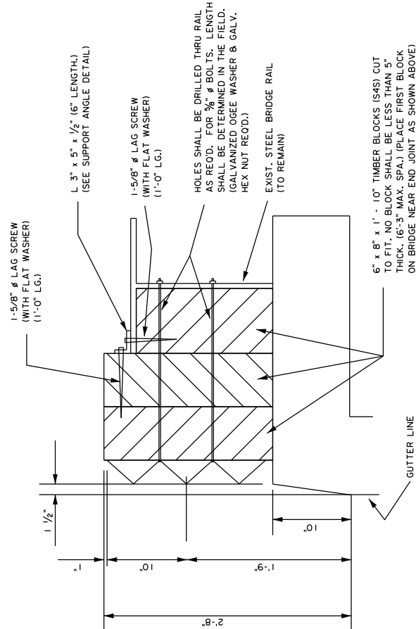
STEEL BRIDGE RAIL BLOCK OUT DETAIL NOT TO SCALE
