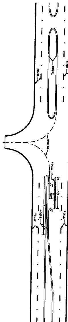
5 LANE - Major Intersection (Left Turn Lane Provided)
