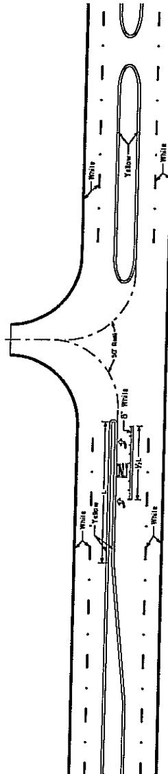
4 LANE DIVIDED
