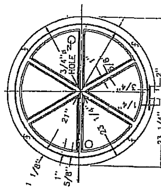
TOP VIEW OF MANHOLE COVER
