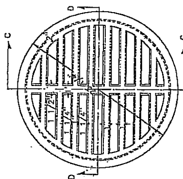
TOP VIEW OF OPEN GRATE MANHOLE COVER
