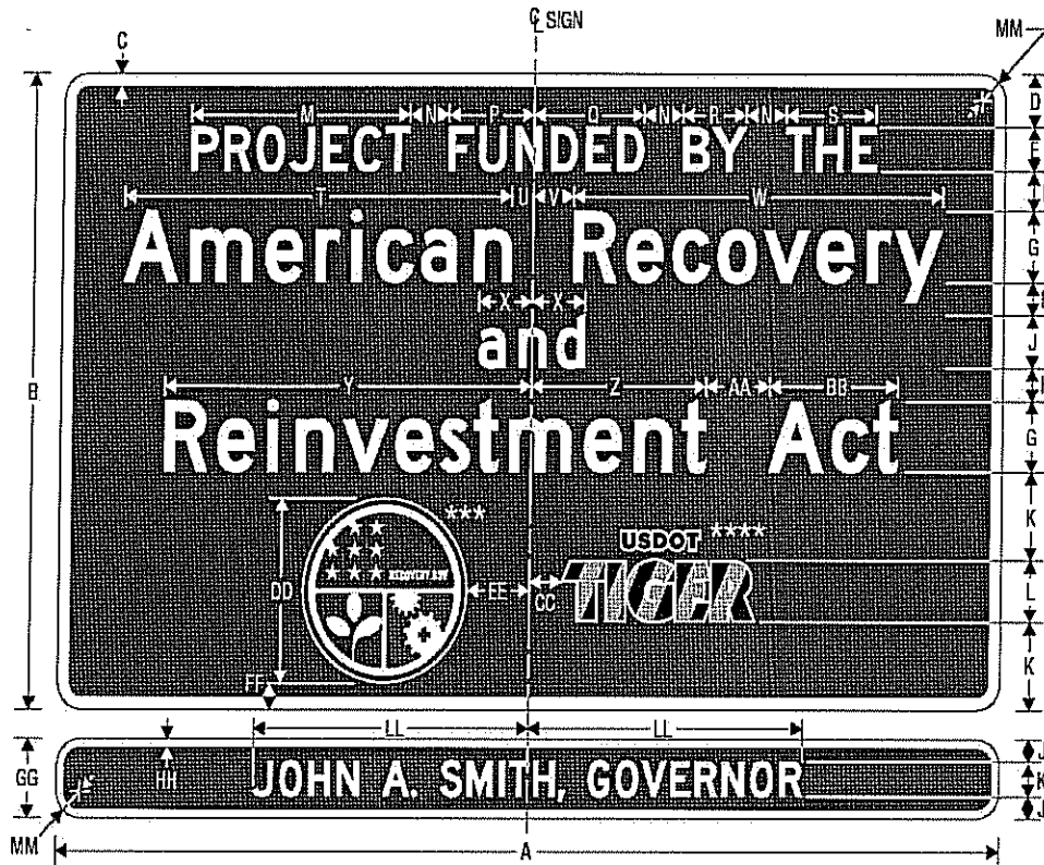
PROJECT FUNDING SOURCE SIGN AND OPTIONAL SUPPLEMENTAL PLAQUE
