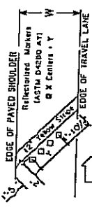
DETAIL OF INSIDE SHOULDER MARKINGS IN ADVANCE OF AND ON NARROW BRIDGES
