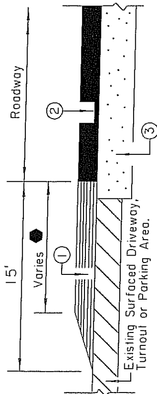
SURFACING DETAIL (SECTION H-H)
