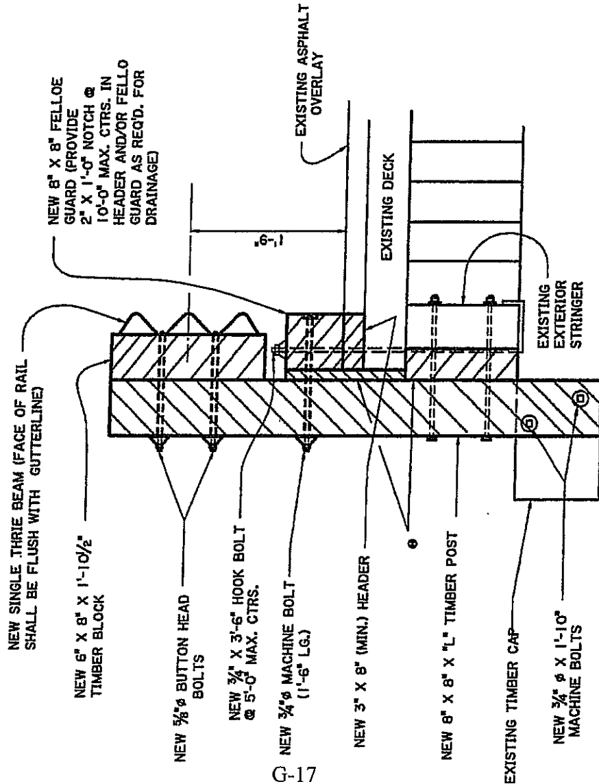
TYPICAL SECTION
