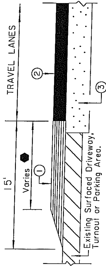
SURFACING DETAIL (SECTION H-H)
